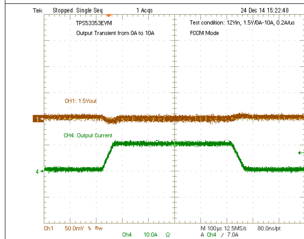
Figure 46. Output Transient with FCCM Mode
