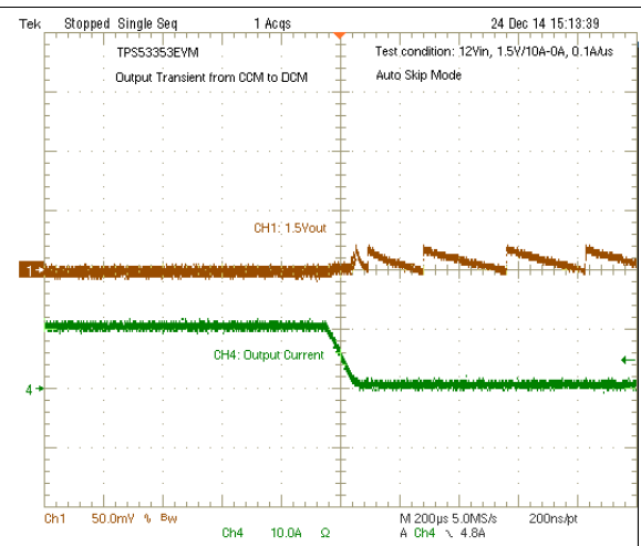
Figure 45. Output Transient from DCM to DCM
