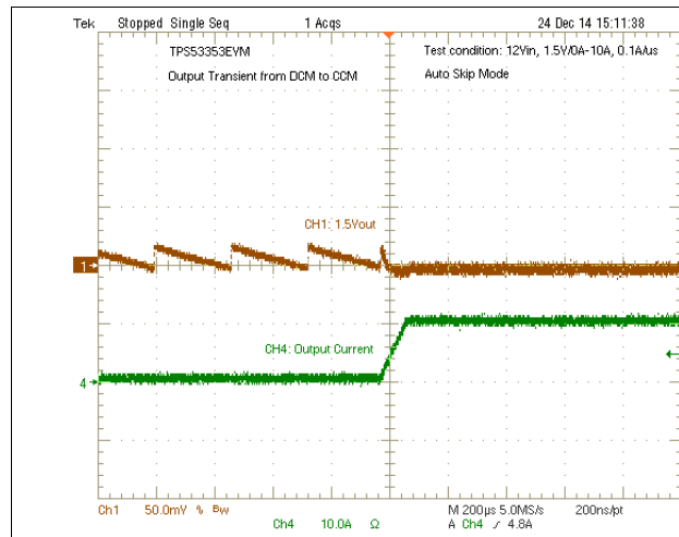
Figure 44. Output Transient from DCM to CCM
