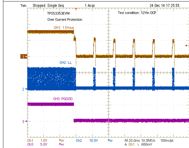
Figure 48. Output Overcurrent Protection
