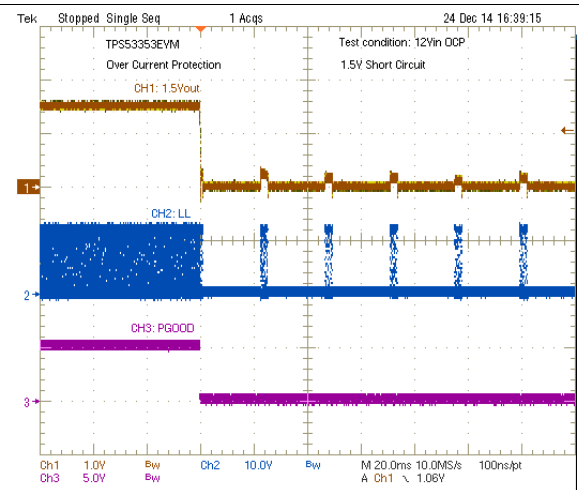
Figure 49. Output Short-Circuit Protection
