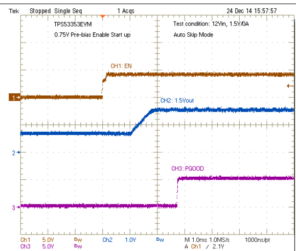
Figure 47. Output 0.75-V Prebias Turnon
